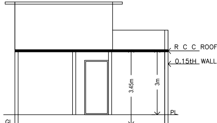
SECTION @ X-X
